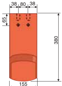
Bobrovec zračnik 15,5/38 Berlinski bobrovec
