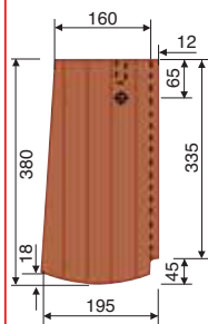
1 1/4 krajnik desni 19,5/38 Berlinski bobrovec
