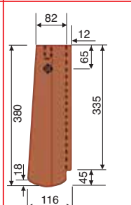
3/4 krajnik desni 11,6/38 Berlinski bobrovec
