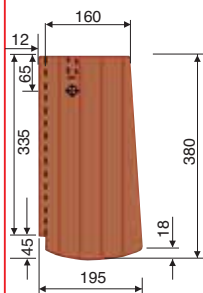
1 1/4 krajnik levi 19,5/38 Berlinski bobrovec
