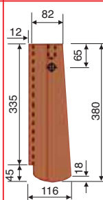
3/4 krajnik levi 11,6/38 Berlinski bobrovec
